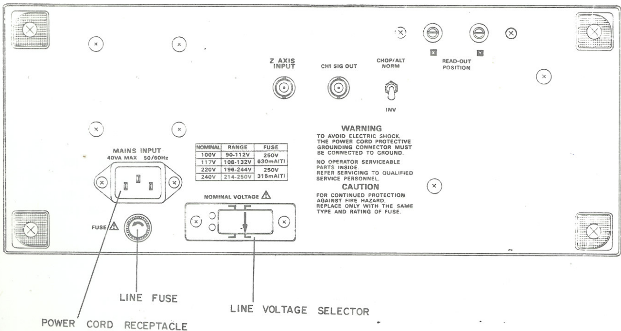
Fig. 1 LINE VOLTAGE SELECTOR
