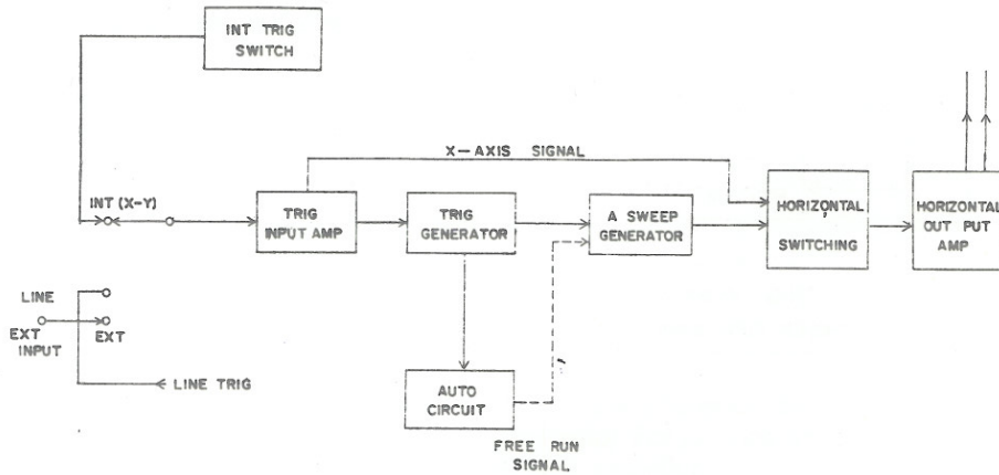
Fig. 4 HORIZONTAL DEFLECTION UNIT
