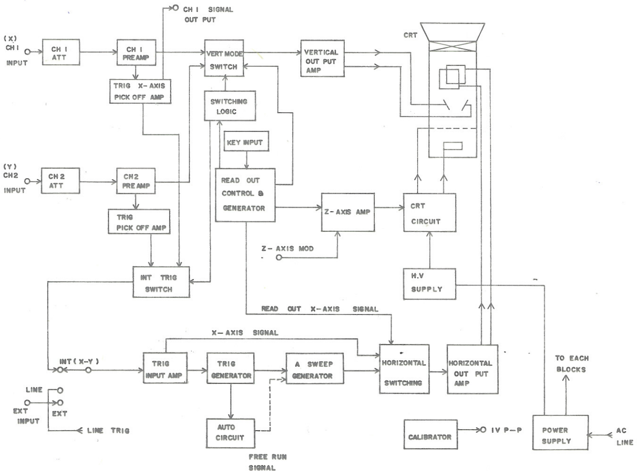
Fig. 2 OVERALL BLOCK DIAGRAM
