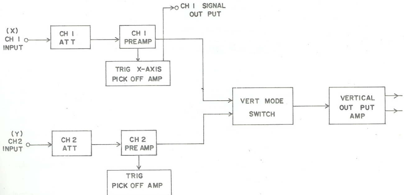
Fig. 3 VERTICAL DEFLECTION UNIT
