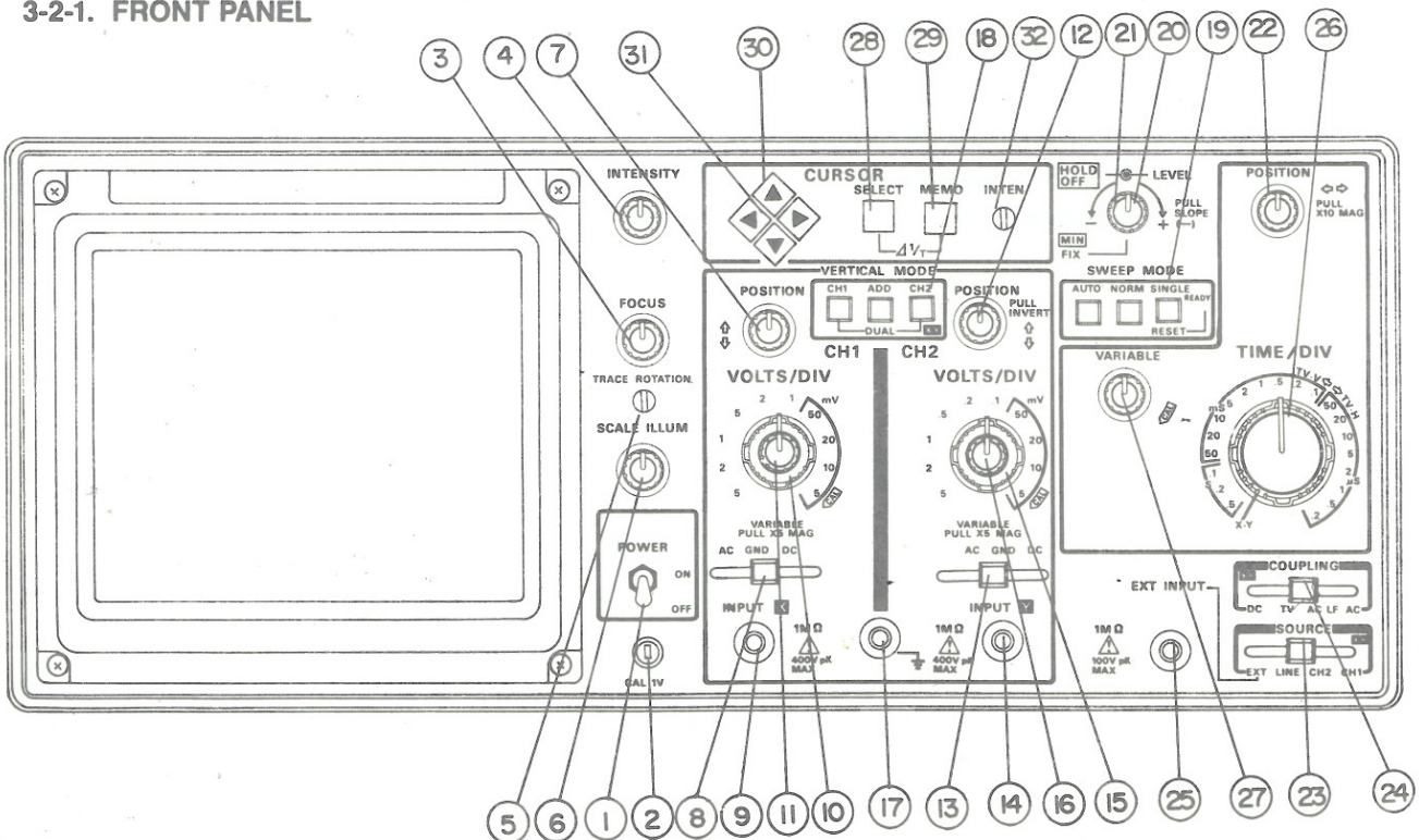
Fig. 8 FRONT PANEL
